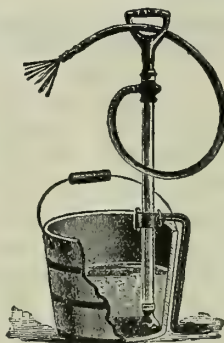
Success Pump
